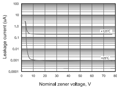
Fig.5 Typical leakage current
